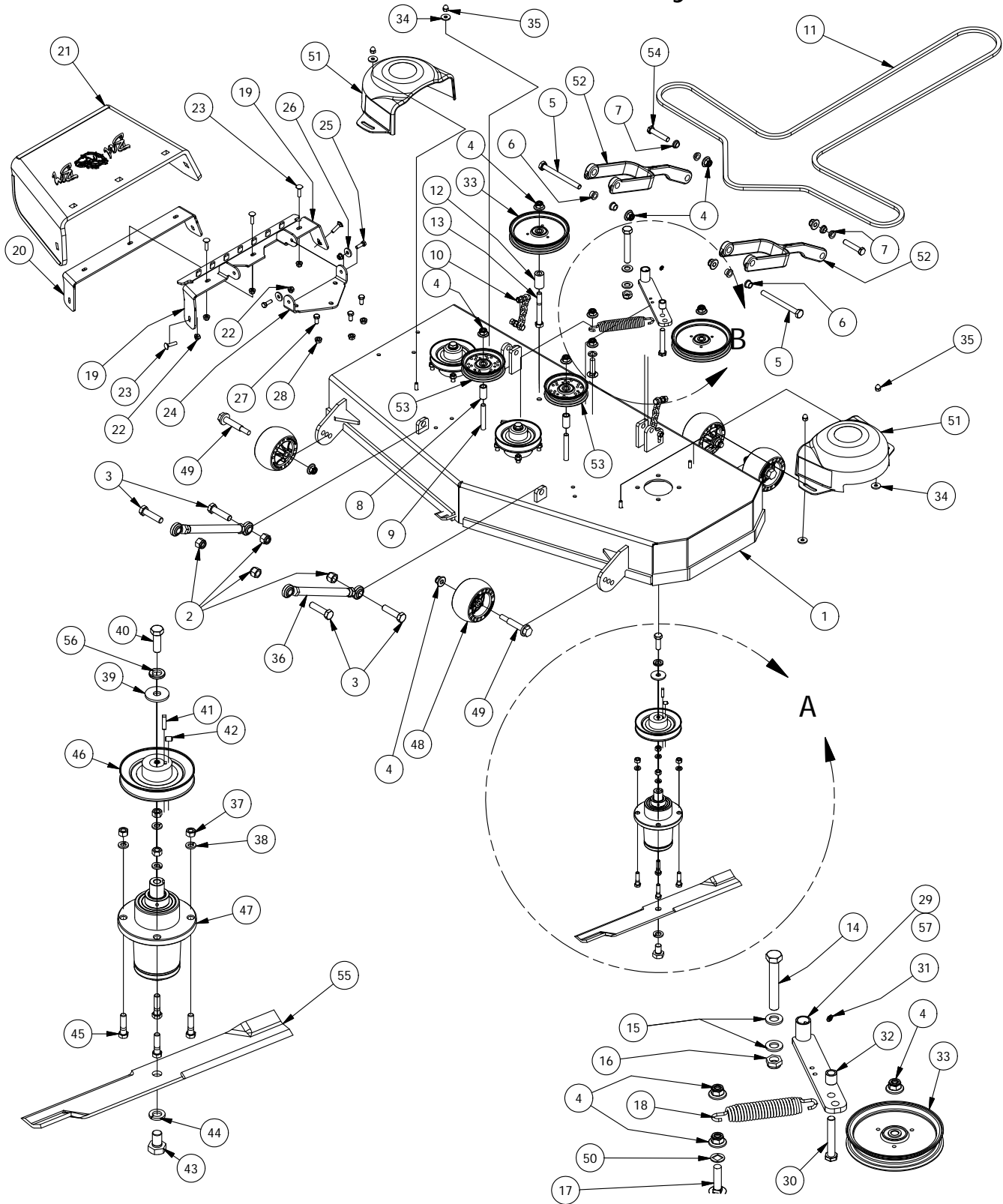
DETAIL A
